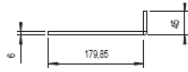
Universal mounting plate
